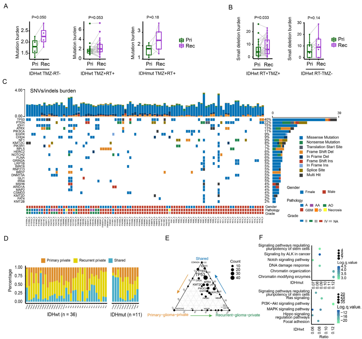
Fig. 1. The landscape of driver mutations in paired primary and recurrent gliomas. (A) The boxplots depicted the mutation burden between primary and TMZ-untreated/ TMZ-treated/ glioma samples. A two-sided paired t -test was applied for statistical testing. (B) The boxplots depicted the small-deletion burden between primary and TMZ-untreated/ TMZ-treated/ radiated GBM samples. A two-sided paired t -test was applied for statistical testing. (C) Oncoprint of functional driver mutations in 97 glioma samples. The upper stacked bar plots illustrate the total number of SNVs and indels in each sample. (D) The proportion of SNVs/indels that are shared, primary-private, or recurrent-private. (E) Ternary plot of mutation counts of driver genes in shared, primary-private, and recurrent-private mutation. (F) Recurrent-private driver mutations were used for pathway enrichment analysis. The Y-axis label represents the pathway, and X-axis label represents the gene term ratio (gene term ratio = gene numbers annotated in this pathway term/ all gene numbers annotated in this pathway term). The bubble size represented the number of genes enriched in the pathway, and color showed the -\log(q\text{-value}) of the enriched pathway. RT: Radiotherapy; TMZ: Temozolomide; Pri: Primary gliomas; Rec: Recurrent gliomas.
